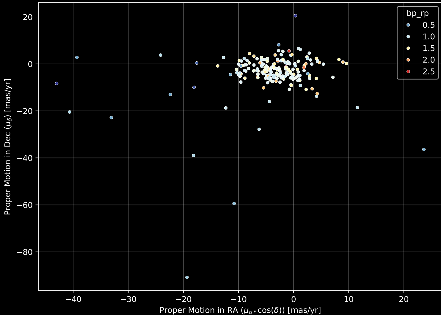
APOGEE DR17 Field: [330+50_btx] Proper Motion Diagram (n= 209)
