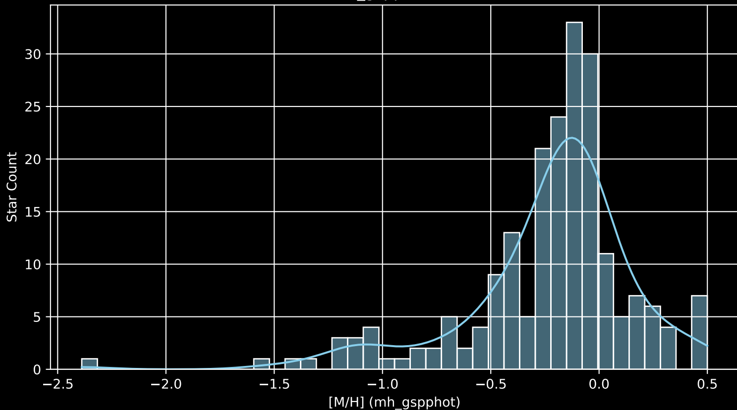
APOGEE DR17 Field: [330+50_btx [M/H] (mh_gspphot) (n= 206)
