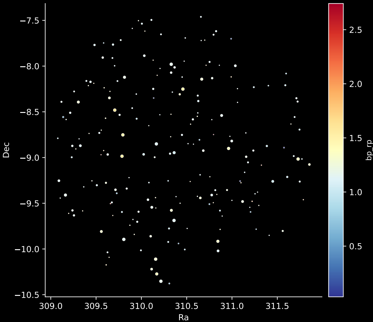
APOGEE DR17 Field: [330+50_btx] Stars: 209
