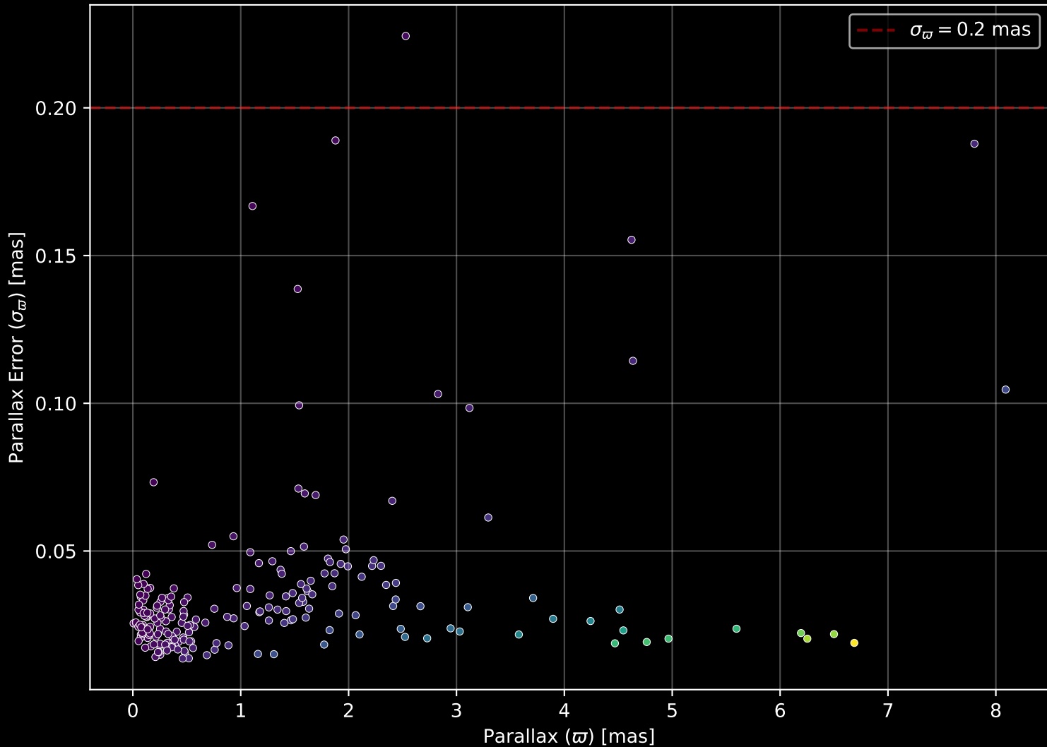
APOGEE DR17 Field: [330+50_btx] Parallax Quality (n= 209)
