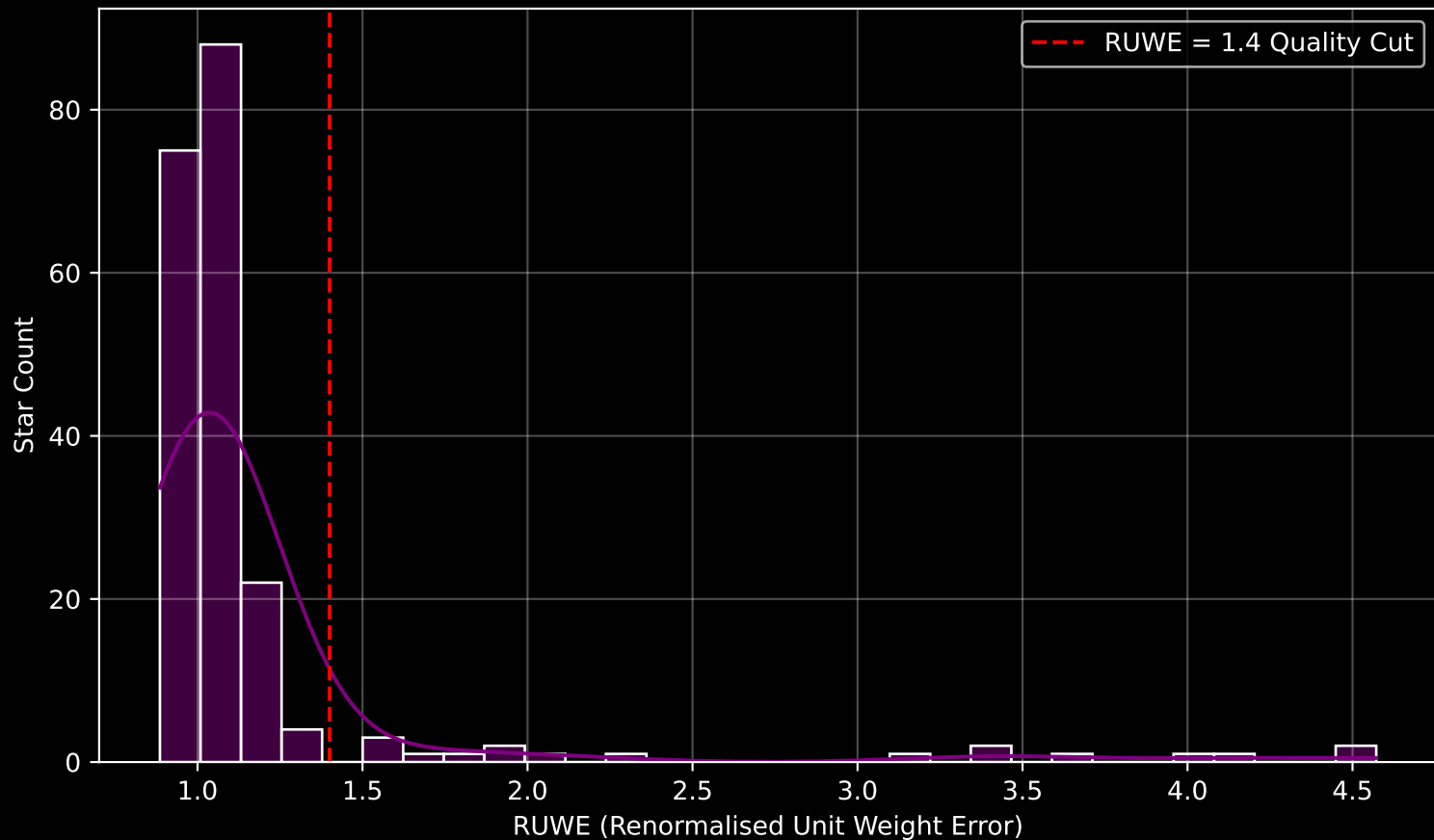
GAPOGEE DR17 Field [330+50_btx] RUWE Distribution (n= 206)
