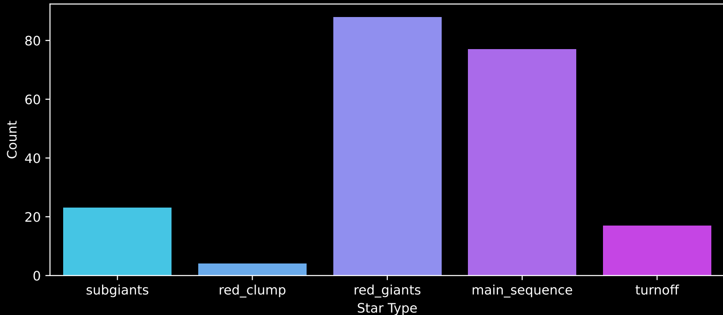
APOGEE DR17 Field: [330+50_btx] Count plot of Star Type
